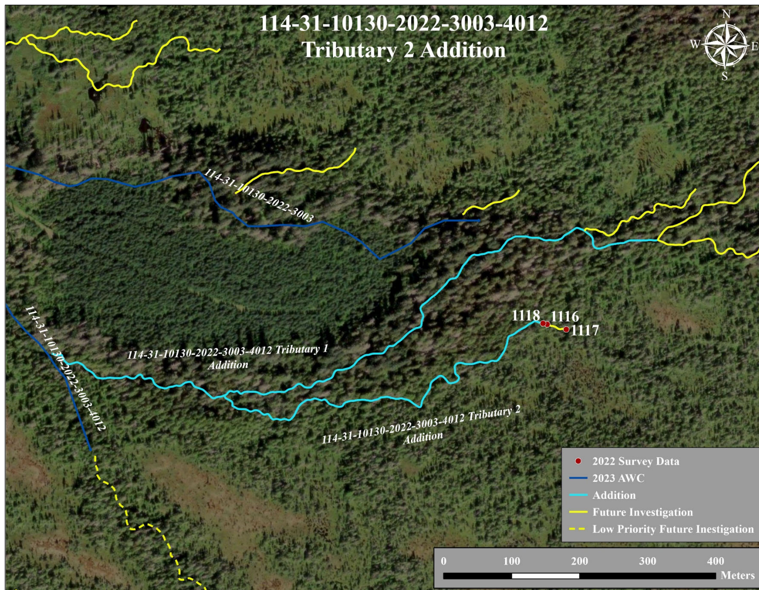
Figure 4.–114-31-10130-2022-3003-4012 tributary 2 addition map.
